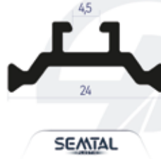
PVC ISI BARIYERİ 24 mm PVC Thermal Barrier 24 mm SPVB-022
